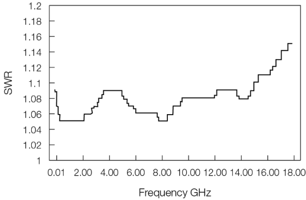
Typical SWR, 10 MHz to 18 GHz (25 °C \pm 10 °C) for E9300A and E9301A sensor.
