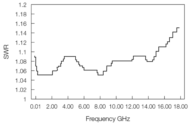
Typical SWR, 10 MHz to 18 GHz ( 25^{\circ}\text{C} \pm 10^{\circ}\text{C} ) for E9300A and E9301A sensor.
