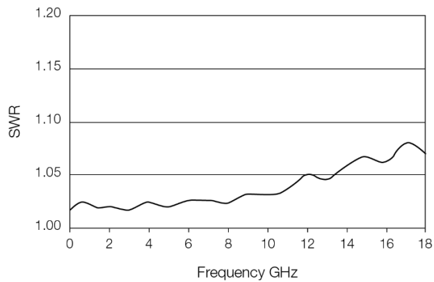
Typical SWR, 10 MHz to 18 GHz ( 25^{\circ}\text{C} \pm 10^{\circ}\text{C} ) for E9300B and E9301B sensors.
