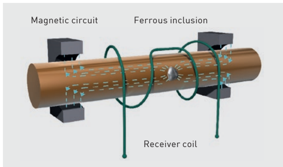
The principle behind ferritic inclusion detection
