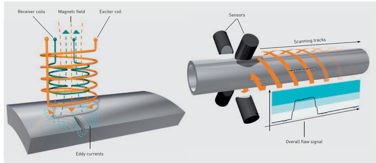
How eddy current testing works with rotating sensors
