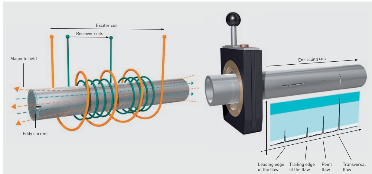
How eddy current testing works with an encircling test coil
